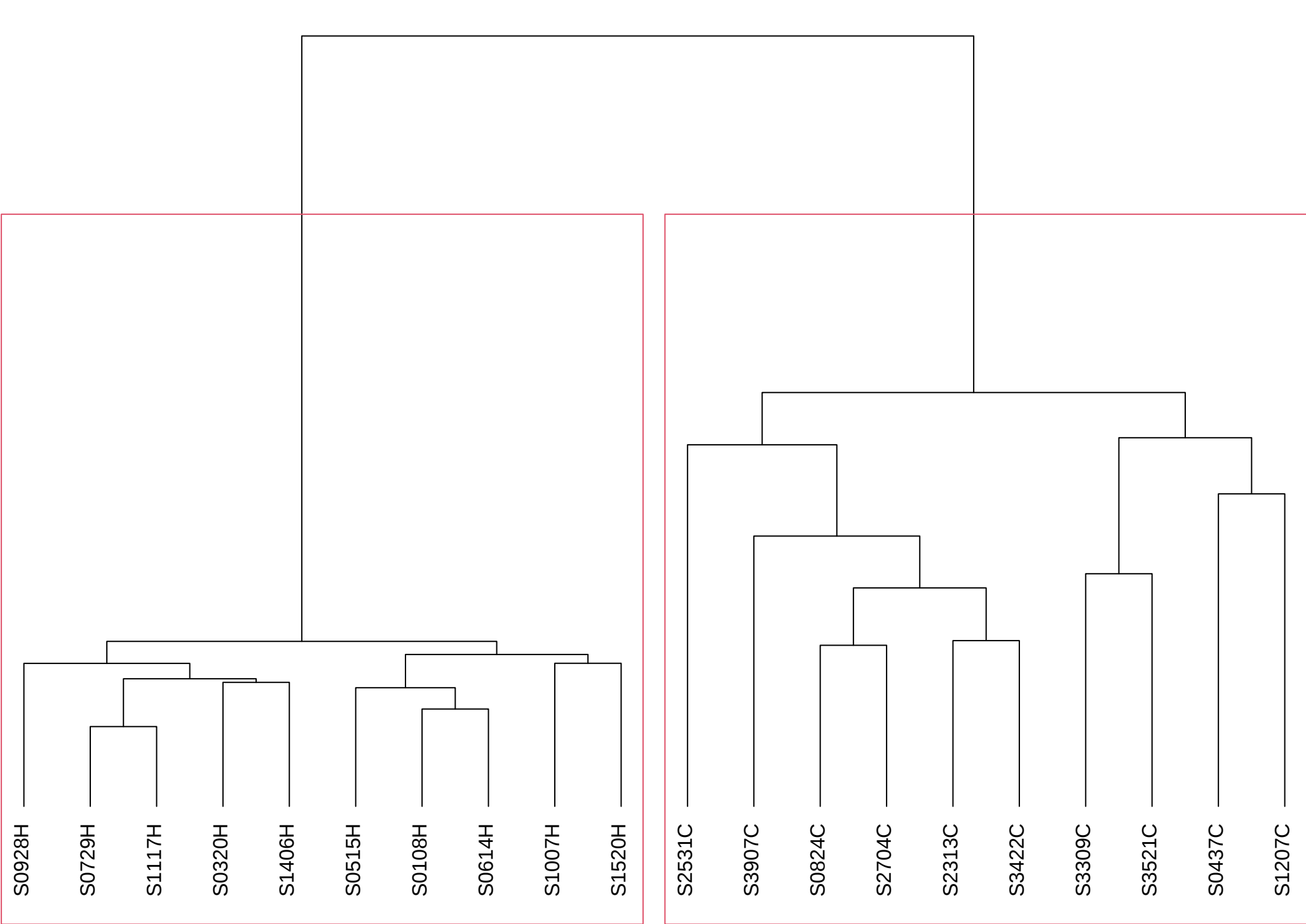
Cluster Dendrogram
