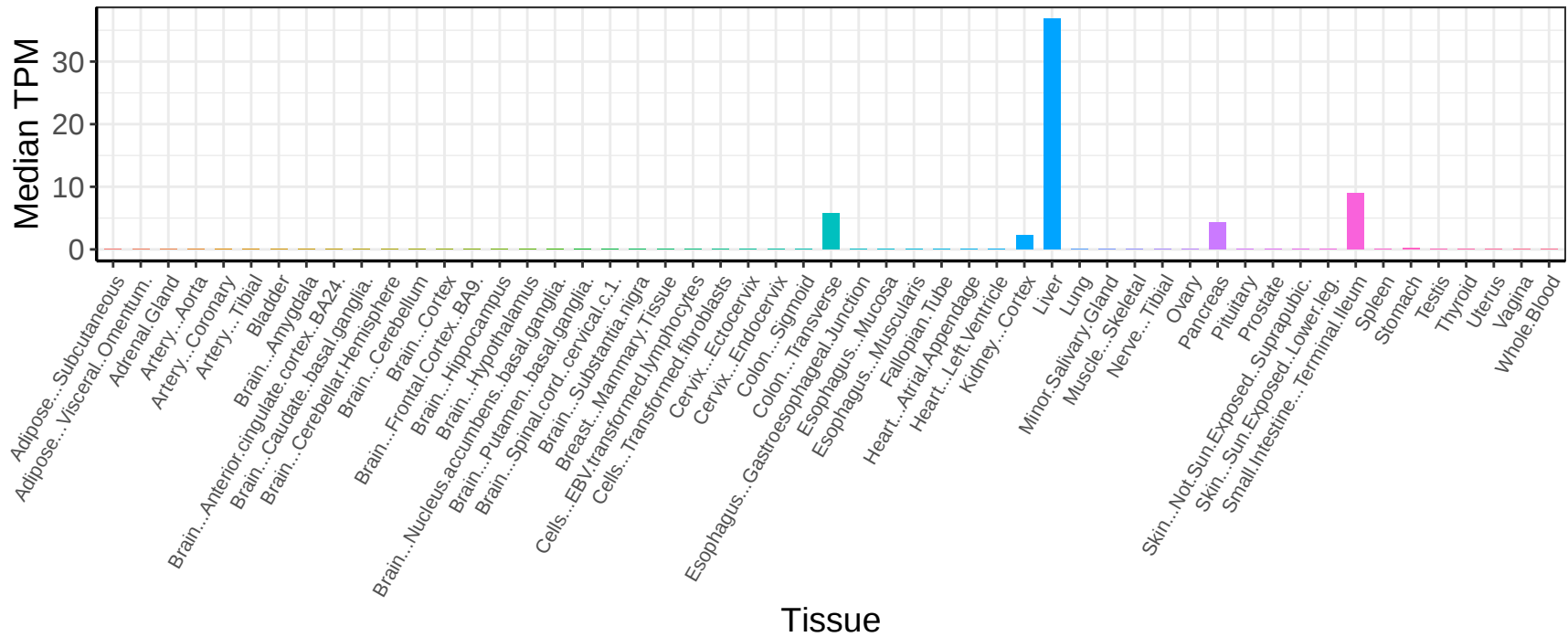
A1CF Expression Profile (GTEx)
