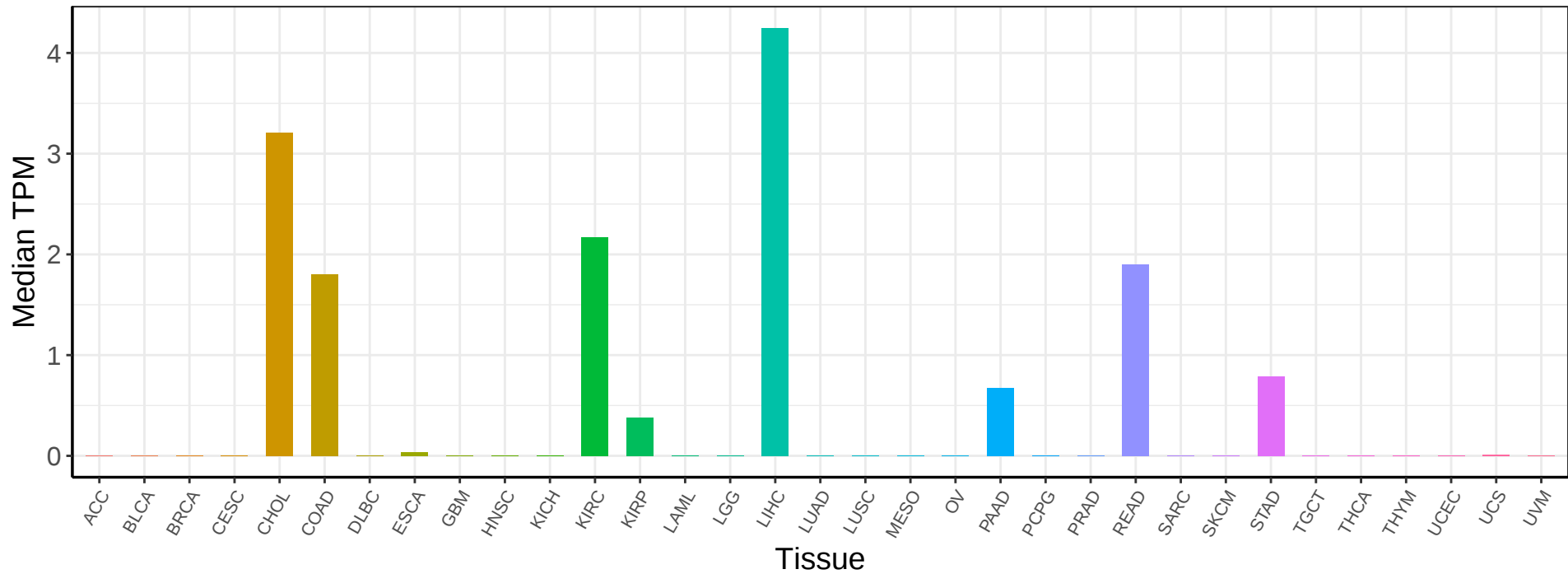
A1CF Expression Profile (TCGA Pan-cancer)
