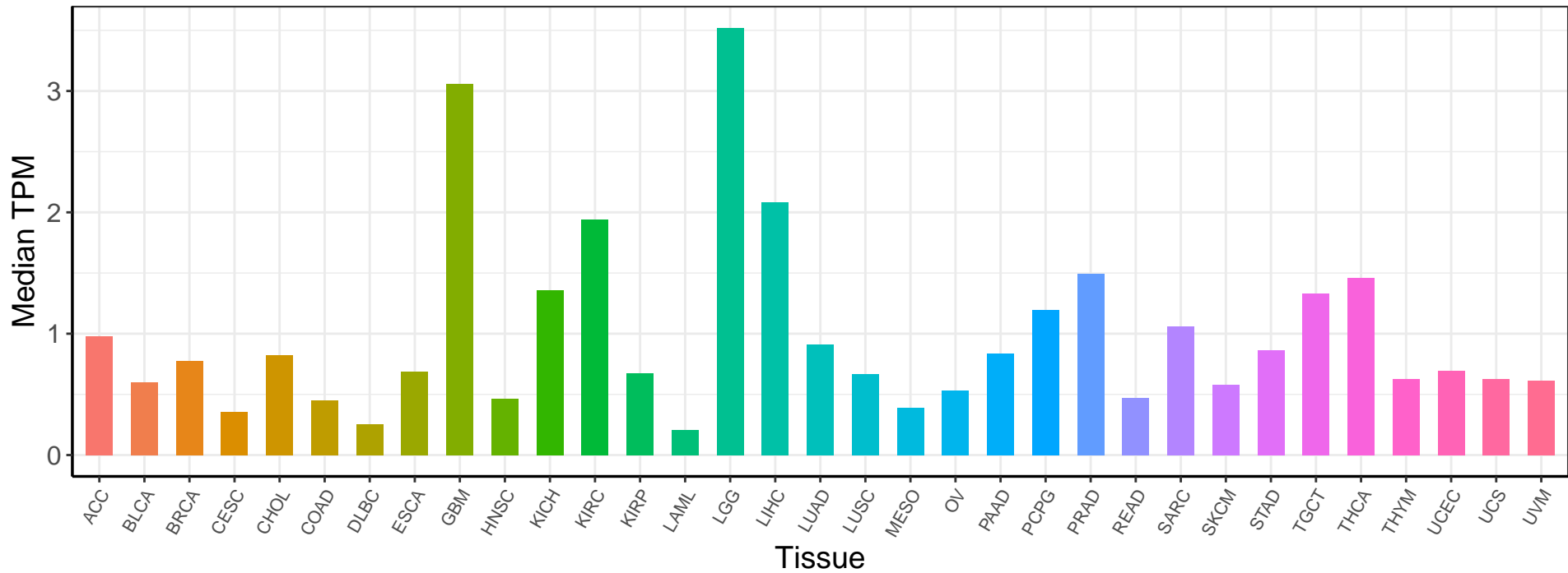
ABCG2 Expression Profile (TCGA Pan-cancer)
