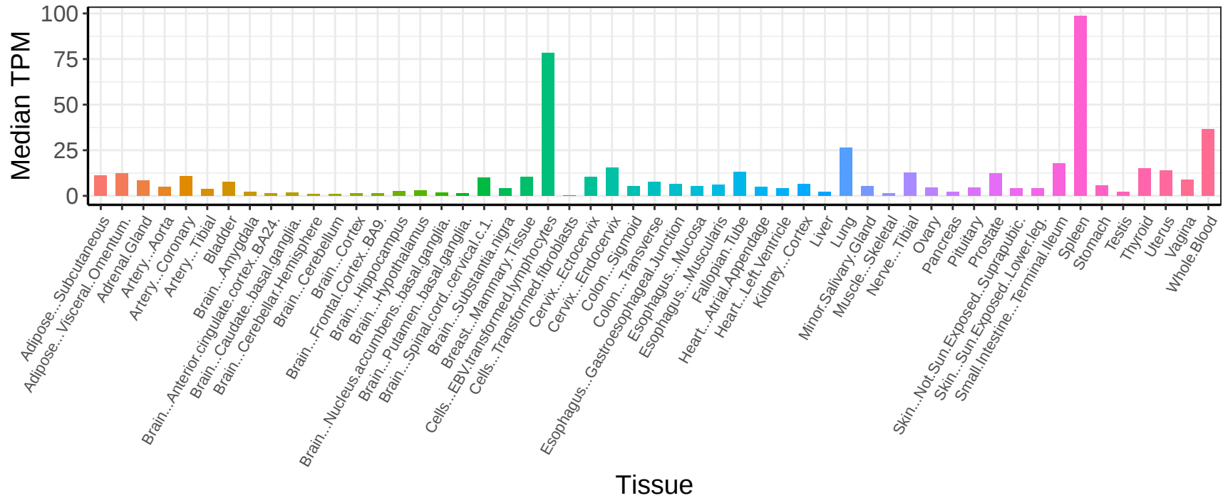
ABI3 Expression Profile (GTEx)
