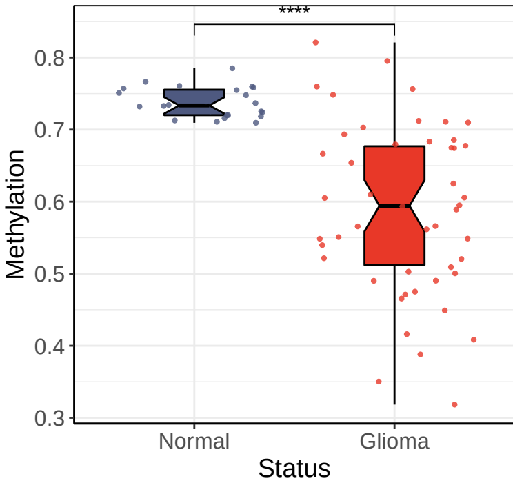
ABI3 promoter (GSE50923 Dataset)
