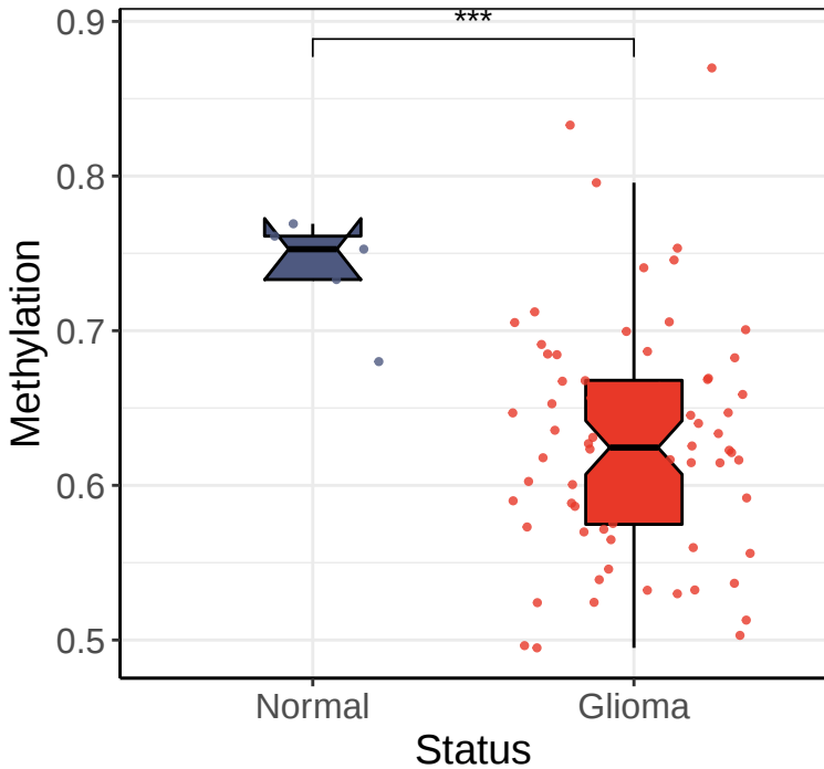
ANO7 promoter (GSE60274 Dataset)
