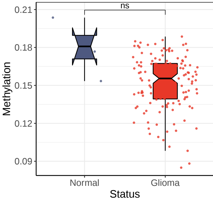
ATF5 promoter (GSE36278 Dataset)
