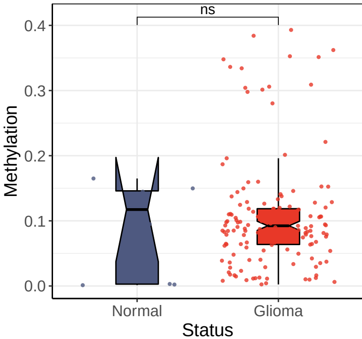
BCL2L1 promoter (CGGA Dataset)
