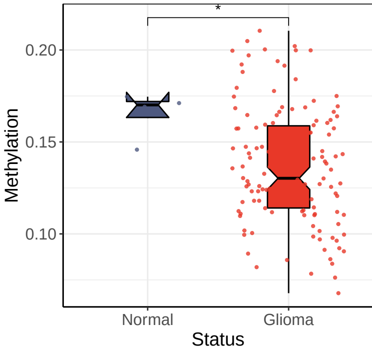
BCL2L1 promoter (GSE36278 Dataset)
