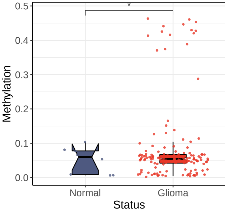
BCL2L12 promoter (CGGA Dataset)
