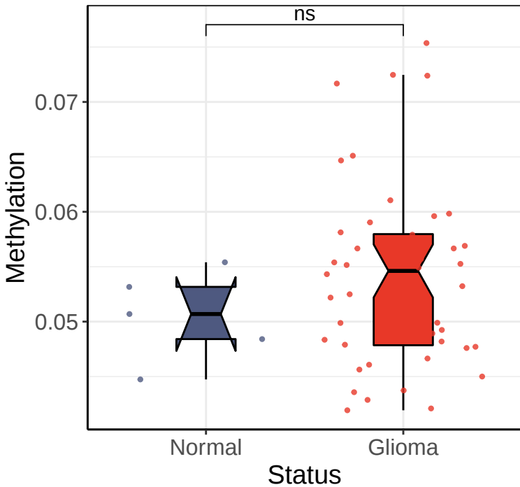
BCL6 promoter (GSE61160 Dataset)
