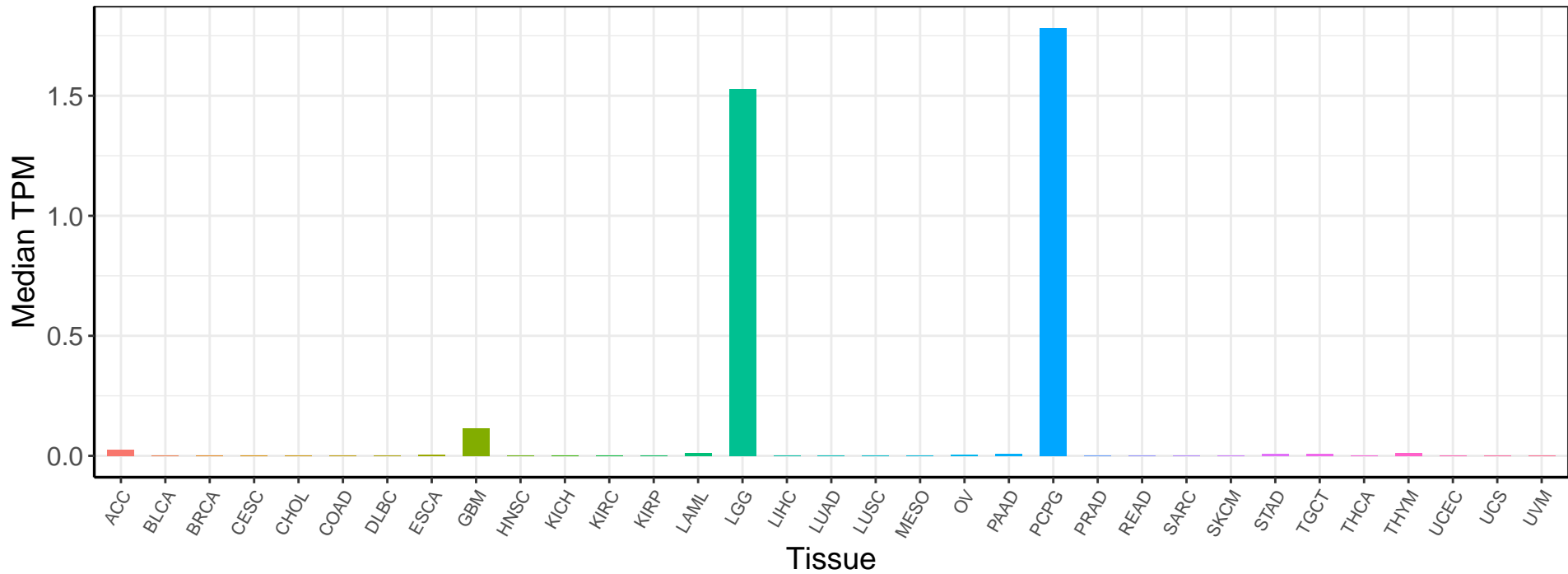
CACNG2 Expression Profile (TCGA Pan-cancer)
