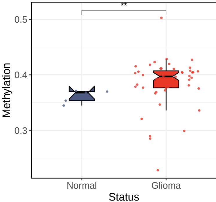
CACNG3 promoter (GSE61160 Dataset)
