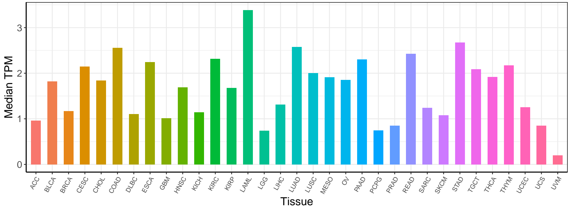
CASP10 Expression Profile (TCGA Pan-cancer)
