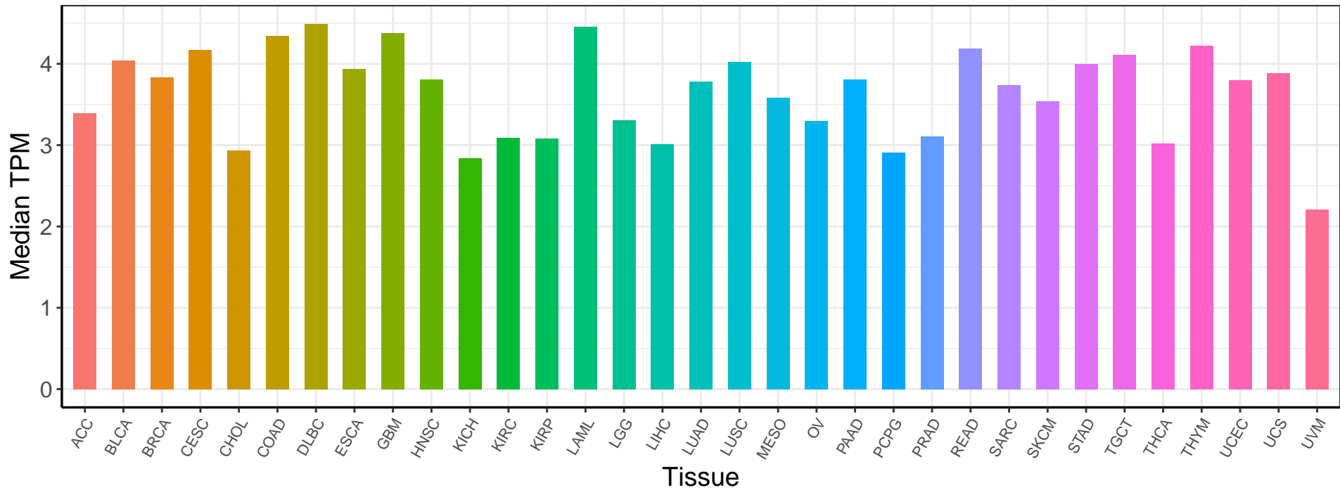
CASP3 Expression Profile (TCGA Pan-cancer)
