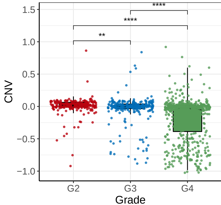
CHEK2 (TCGA Dataset)
