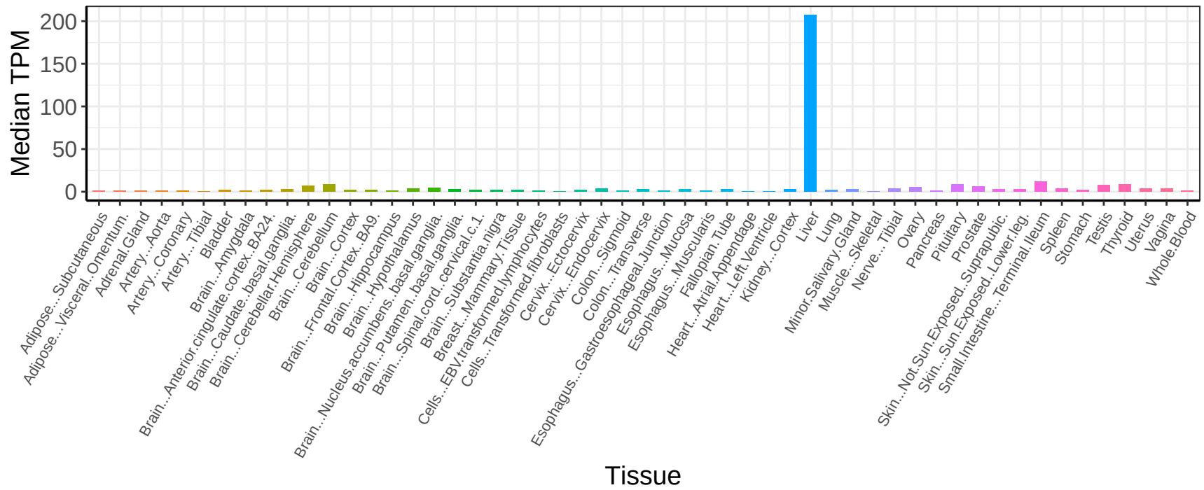
CYP2D6 Expression Profile (GTEx)
