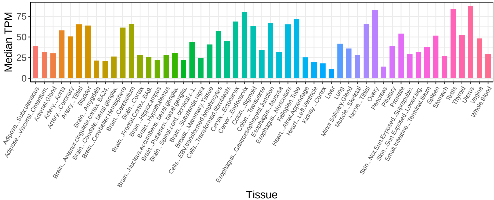
DPF2 Expression Profile (GTEx)
