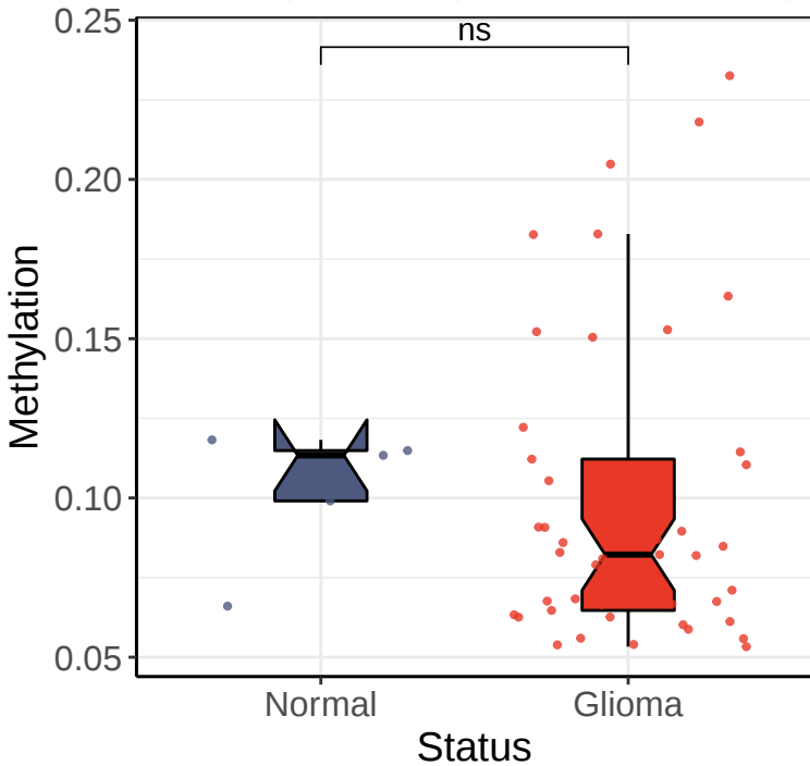
FGFR1 promoter (GSE61160 Dataset)
