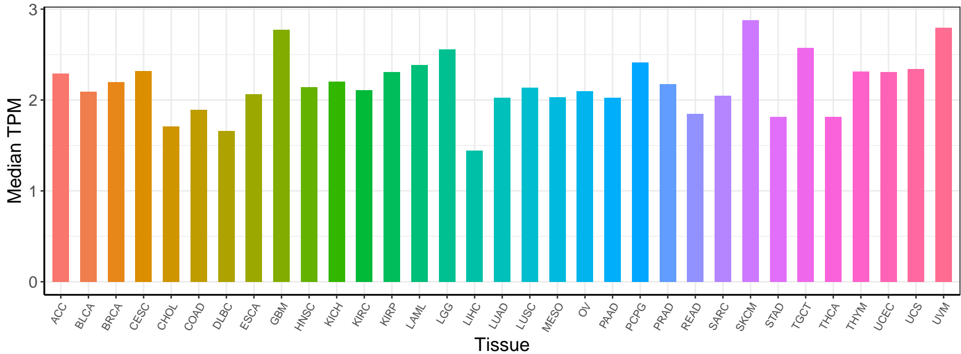
FNTB Expression Profile (TCGA Pan-cancer)
