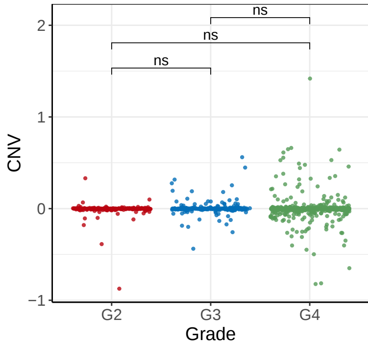
IL1B (TCGA Dataset)
