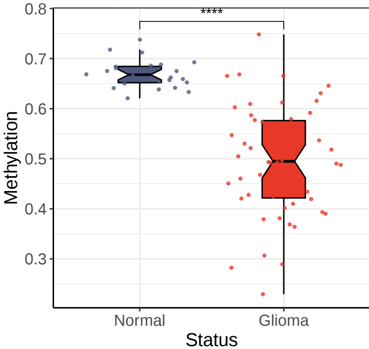
IL1B promoter (GSE50923 Dataset)
