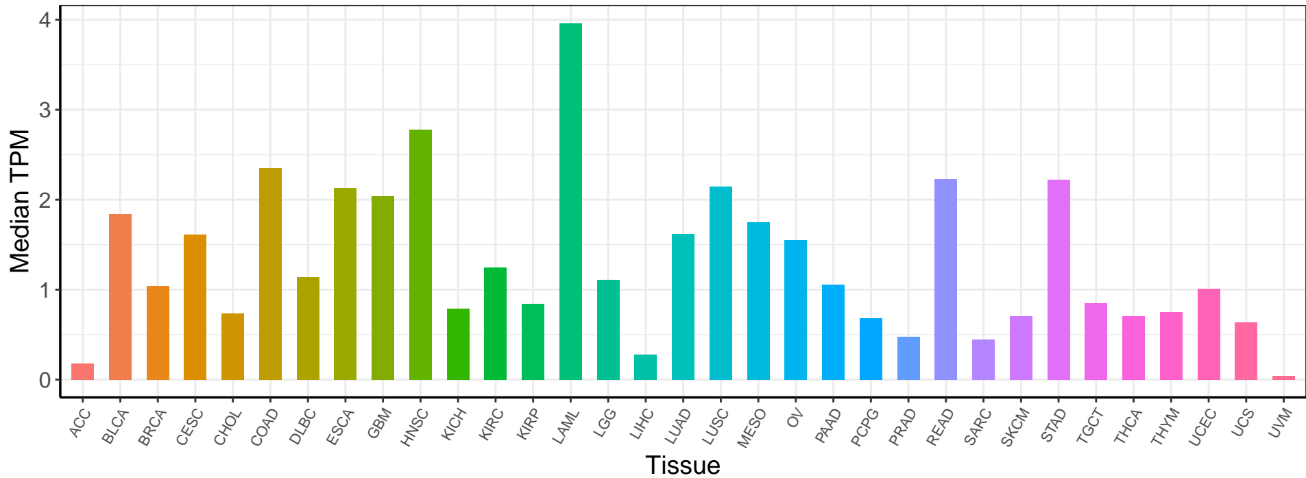
IL1B Expression Profile (TCGA Pan-cancer)
