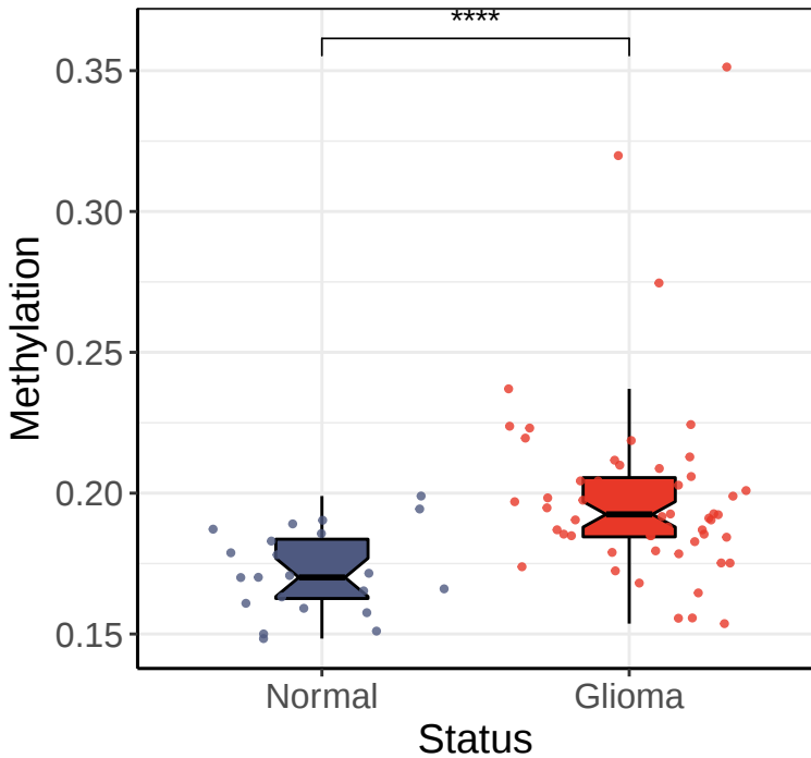
PPAT promoter (GSE50923 Dataset)
