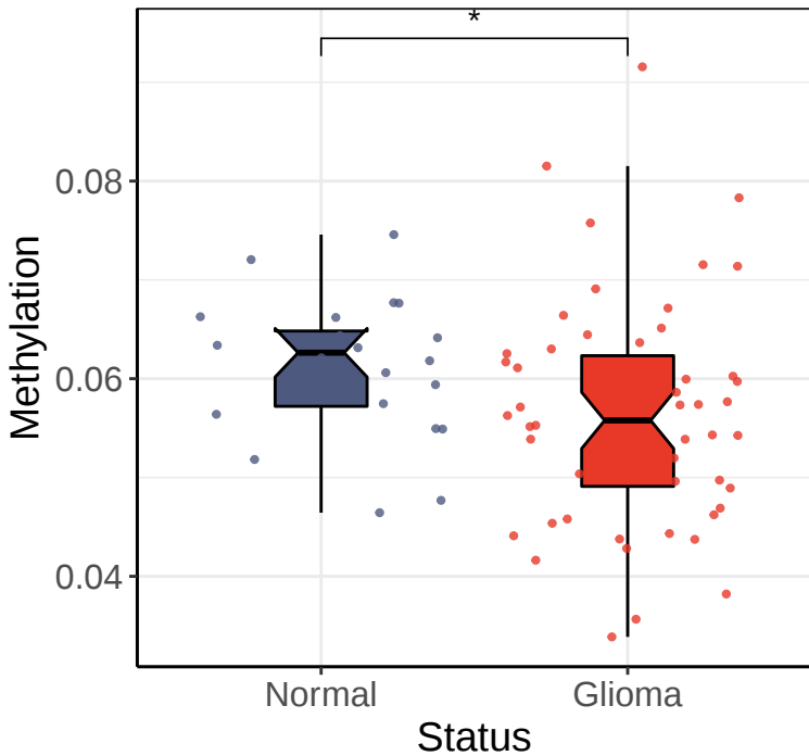
PTPN11 promoter (GSE50923 Dataset)
