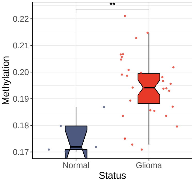
RB1 promoter (GSE61160 Dataset)
