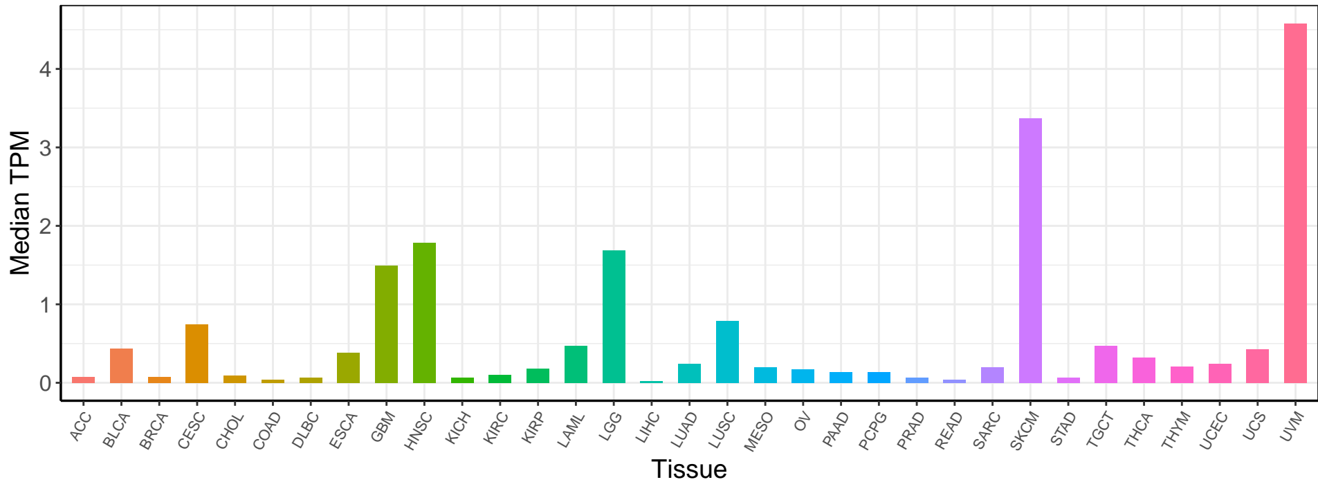
RGS20 Expression Profile (TCGA Pan-cancer)
