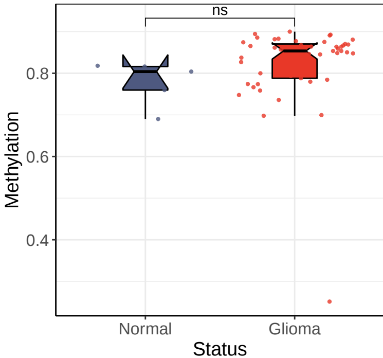
SFN promoter (GSE61160 Dataset)
