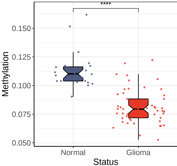
SLC2A3 promoter (GSE50923 Dataset)
