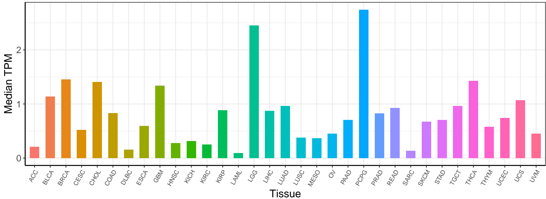
SRCIN1 Expression Profile (TCGA Pan-cancer)
