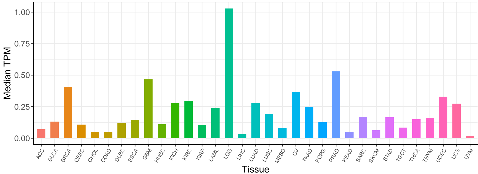
TACR1 Expression Profile (TCGA Pan-cancer)
