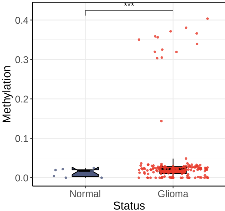
hsa-mir-320 promoter (CGGA Dataset)
