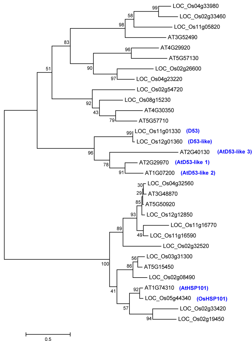
Extended Data Figure 3 | Phylogenetic tree of D53-like family proteins in rice and Arabidopsis . BlastP was done using the D53 protein sequence against all rice and Arabidopsis proteins at the MSU Rice Genome Annotation Project. In the BlastP result, rice proteins were filtered using cut-off E value < 0.1 plus top query coverage > 10% and Arabidopsis proteins were filtered using
