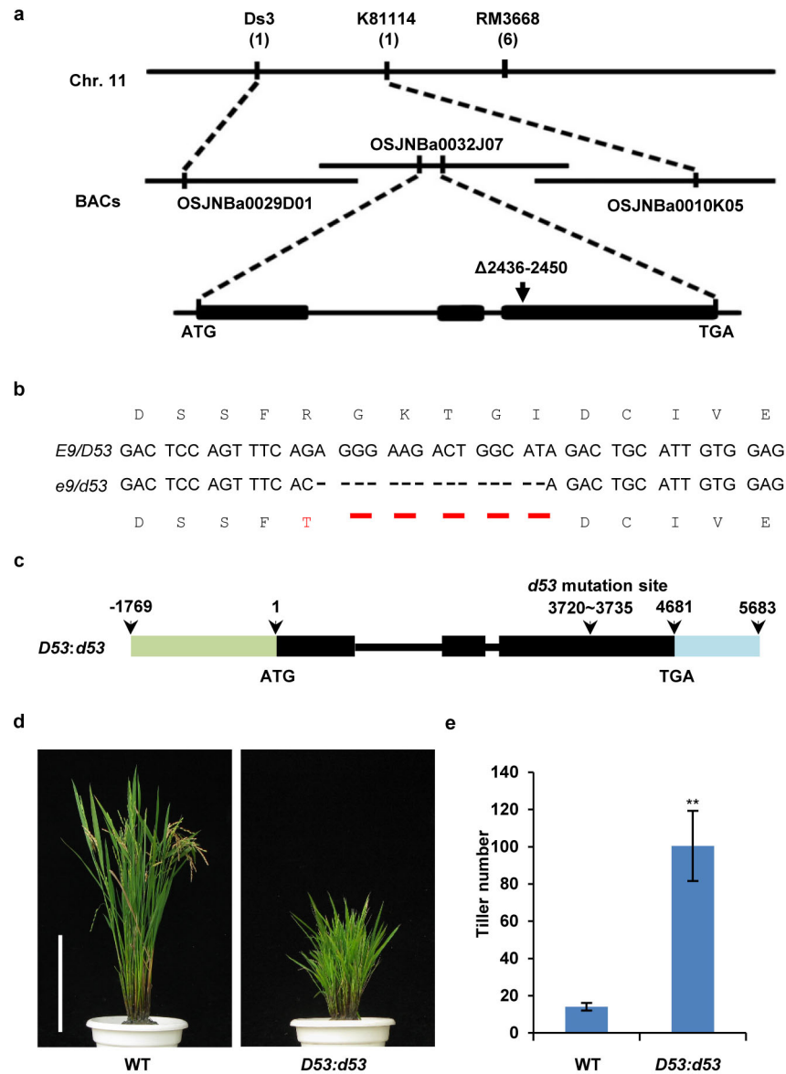
Extended Data Figure 2 | Cloning and confirmation of E9/D53 . a , E9 was mapped in the interval between molecular markers Ds3 and K81114 on chromosome 11 using 142 recessive individual plants showing normal tillering phenotype from an F_2 population. Numbers under the markers indicate recombinants. b , E9/D53 mutation sites in e9/d53 in the coding region and its amino acid changes. c , Schematic diagram of D53:d53 constructs. d , Phenotypes of wild-type and D53:d53 transgenic plants at the mature stage.
