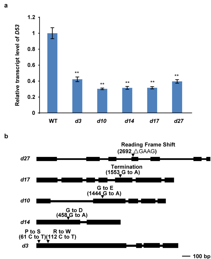
Extended Data Figure 5 | D53 expression levels in d mutants and the mutation sites in other d mutants used in this study. a , Expression levels of D53 revealed by qPCR in wild-type, d3 , d10 , d14 , d17 and d27 seedlings.
