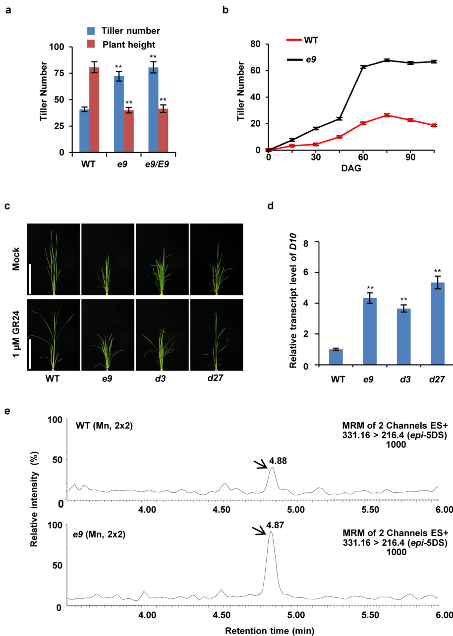
Extended Data Figure 1 | Characterization of the e9 mutant. a , Tiller number and plant height of wild-type, homozygous and heterozygous e9 plants at the heading stage. Values are means \pm s.d. ( n = 8 ). The double asterisks represent significant difference determined by the Student's t -test at P < 0.01 . b , Kinetic comparison of tiller numbers between wild-type and e9 plants at different developmental stages. Values are means \pm s.d. ( n = 8 ). DAG, days after germination. Rice plants ( a and b ) were cultivated in the field in Beijing in the natural growing season. c , Four-week-old seedlings of wild-type, e9 , d3 and
