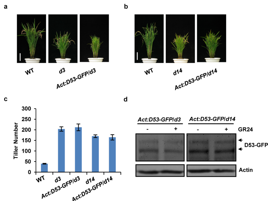
Extended Data Figure 8 | Phenotypes of transgenic plants of constitutively expressed D53-GFP in d3 and d14 . a , Phenotypes of wild-type, d3 and Act:D53-GFP/d3 transgenic plants at the mature stage. Scale bar, 10 cm. Six independent transgenic lines showed similar phenotypes. b , Phenotypes of wild-type, d14 and Act:D53-GFP/d14 transgenic plants at the mature stage. Scale bar, 10 cm. Six independent transgenic plants showed similar phenotypes.
