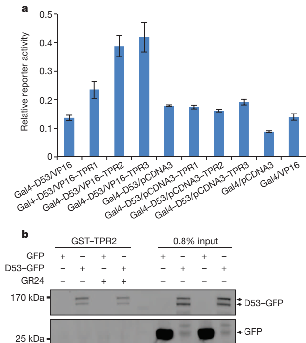
Figure 4 | Interaction of D53 with TPR proteins. a , Mammalian two-hybrid assays showing interaction of D53 with TPR proteins. Values are means \pm s.d. of three independent experiments. VP16, herpes simplex virus virion protein 16. b , Pull-down assay for GST-TPR2 and lysates of Act:D53-GFP calli in the absence or presence of 10 \mu M GR24. D53 –GFP and GFP were detected with the monoclonal anti-GFP antibody.
