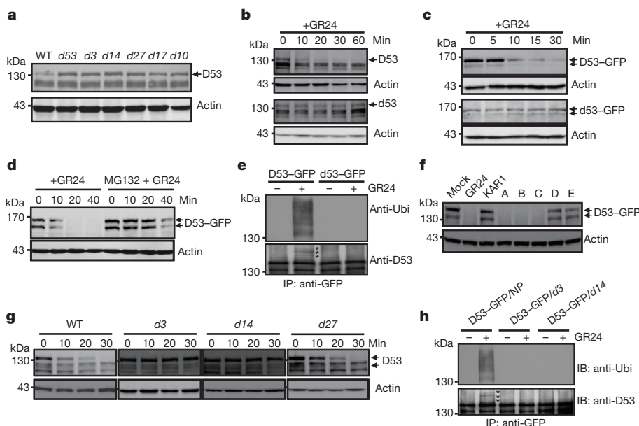
Figure 2 | SL-induced D53 degradation by the ubiquitin proteasome system. a , Protein levels of D53 in seedlings of wild-type and d mutants detected by immunoblotting with anti-D53 antibodies. b , D53 protein levels in 3-week-old seedlings of the wild type (top) and d53 mutant (bottom) upon 10 \mu M GR24 treatment detected by immunoblotting with anti-D53 antibodies. c , Protein levels of D53-GFP in calli of Act:D53-GFP and Act:d53-GFP transgenic lines at different time points of GR24 (5 \mu M) treatment, as detected by immunoblotting with anti-GFP antibody. d , D53-GFP protein levels at different time points of GR24 treatment (10 \mu M) in the presence or absence of MG132 (50 \mu M), as detected by immunoblotting with anti-GFP antibody. e , Analysis of D53-GFP and d53-GFP ubiquitination in response to GR24 (10 \mu M) treatment. Top, immunoblot with anti-ubiquitin (Ubi) antibody. Bottom, immunoblot with anti-D53 antibodies. Asterisks indicate ubiquitinated D53-GFP proteins. f , D53-GFP protein levels in Act:D53-GFP
