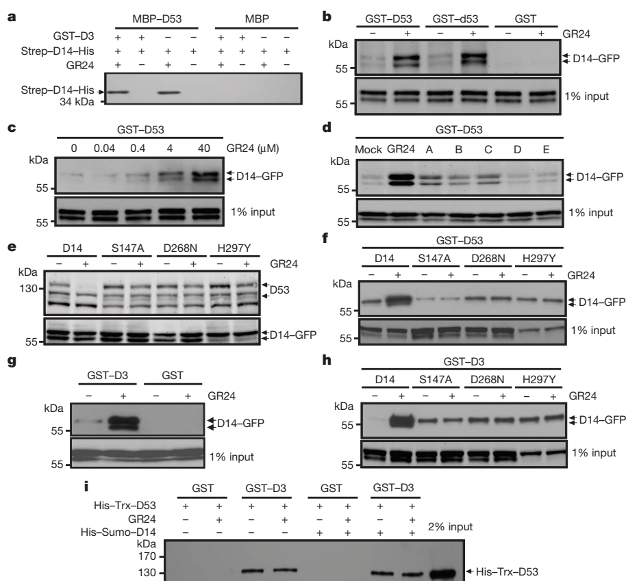
Figure 3 | Interactions among D3, D14 and D53. a , In vitro pull-down assay using maltose-binding protein (MBP)–D53, GST–D3 and Strep–D14–His recombinant proteins in the presence or absence of 10 μM GR24. b , Pull-down assays using recombinant GST–D53 or GST–d53 and lysates prepared from Act:D14-GFP/d14 calli in the absence or presence of 20 μM GR24. c , Pull-down assay using recombinant GST–D53 and lysates prepared from Act:D14-GFP/d14 calli in the presence of GR24 at indicated concentrations. d , Pull-down assay using recombinant GST–D53 and lysates of Act:D14-GFP/d14 calli treated with 20 μM GR24 or SL mimics. e , D53 levels in the 10 μM-GR24-treated calli transformed with D14 mutated at the Ser–His–Asp catalytic triad sites, revealed by immunoblotting with anti-D53 antibodies. D14, Act:D14-GFP/d14 ; S147A, Act:D14(S147A)-GFP/d14 ; D268N, Act:D14(D268N)-GFP/d14 ; H297Y, Act:D14(H297Y)-GFP/d14 . f , Pull-down assay using recombinant GST–D53 and lysates of the calli transformed with D14 mutated at its catalytic triad sites in the absence or presence of 20 μM GR24. g , Pull-down assay using recombinant GST–D3 and lysates of Act:D14-GFP/d14 calli in the absence or presence of 20 μM GR24. h , Pull-down assay using recombinant GST–D3 and lysates of transgenic calli transformed with D14 mutated at its catalytic triad sites in the absence or presence of 20 μM GR24. i , Pull-down assay using recombinant GST–D3 and His–Trx–D53 in the absence or presence of 5 μM GR24 or His–Sumo–D14 recombinant proteins. The D14 recombinant proteins in a were detected with anti-His antibody, GFP-fusion proteins in ( b–d and f–h ) were revealed with anti-GFP antibody, and His–Trx–D53 was detected with anti-D53 antibodies.
