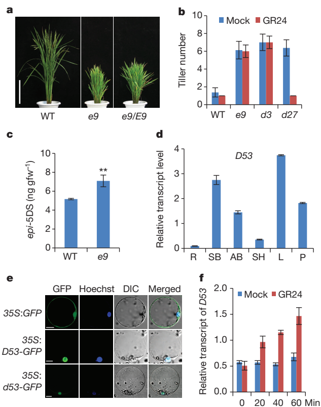
Figure 1 | D53 acts as a negative regulator in SL signalling. a , Phenotypes of e9 mutants. Scale bars, 20 cm. b , Tiller numbers of 4-week-old seedlings of wild-type, e9 , d3 and d27 treated with or without 1 \mu M GR24. Values are means \pm s.d. ( n = 10 ). c , Comparison of epi -5DS contents in wild-type and e9 root exudates. Values are means \pm s.d. ( n = 3 ), **P < 0.01 (Student's t -test). \text{gfw}^{-1} , per gram fresh weight. d , D53 transcript levels in various organs, including roots (R), shoot bases of seedlings (SB), axillary buds (AB), sheaths (SH), young leaves (L) and young panicles (P). Values are means with \pm s.d. of three independent experiments. e , Subcellular localization of 35S::GFP (top), 35S::D53-GFP (middle) and 35S::d53-GFP (bottom) in rice protoplasts. Scale bars, 10 \mu m. f , D53 transcripts upon 20 \mu M GR24 treatment in wild-type seedlings revealed by quantitative (q)PCR. Values are means with \pm s.d. of three independent experiments.
