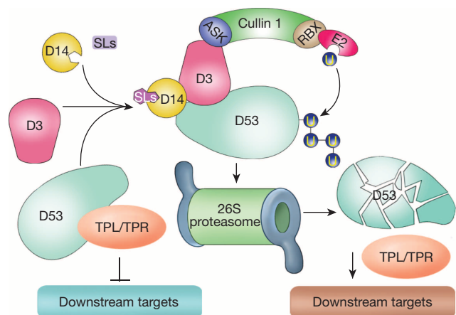
Figure 5 | A proposed model of D53 action. In the absence of SLs, D53 is stable and may recruit TPL/TPR proteins and repress downstream responses. In the presence of SLs, perception of SL leads to SCF D3 -mediated ubiquitination of D53 and its subsequent degradation by the proteasome system, which in turn releases the repression of downstream responses.
