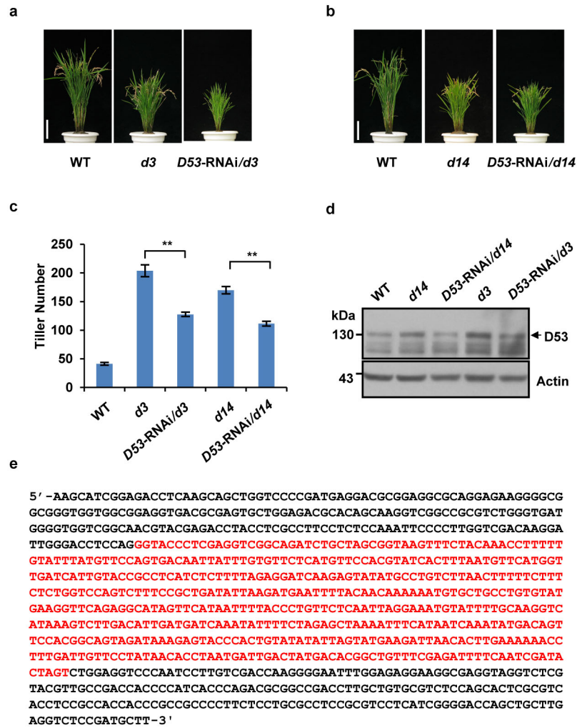
Extended Data Figure 9 | Phenotypes and confirmation of transgenic plants of D53 -RNAi in d3 and d14 . a , Phenotypes of wild-type, d3 and D53 -RNAi/ d3 transgenic plants. Scale bar, 10 cm. Four independent transgenic plants showed similar phenotypes. b , Phenotypes of wild-type, d14 and D53 -RNAi/ d14 transgenic plants at the mature stage. Scale bar, 10 cm. Five independent transgenic plants showed similar phenotypes. c , Tiller numbers of transgenic plants of D53 -RNAi in d3 and d14 backgrounds at the mature stage. Values are
