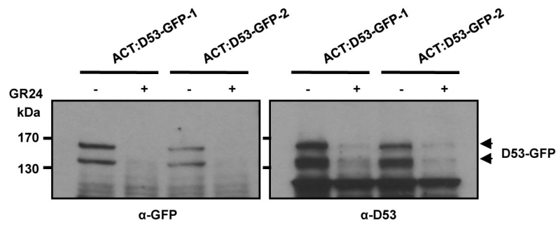
Extended Data Figure 10 | Determination of D53 antibody specificity. Determination of D53 antibody specificity by D53-GFP transgenic calli. Left, anti-GFP (Roche), 1:10,000 dilution; right, anti-D53 (1:10,000).
